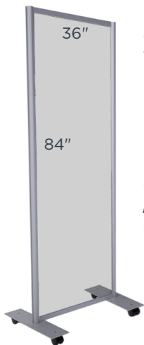
84" Floor Standing Shield with Locking Casters Part# FS-005
